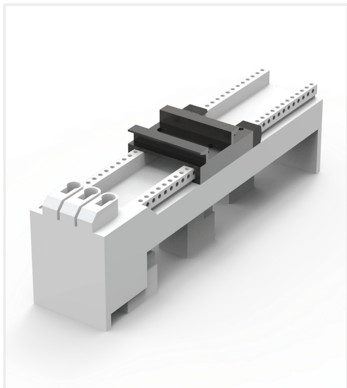
Universal busbar adapter, with one adjustable mounting rail and with spring terminals 1.5-6 mm 2 .
