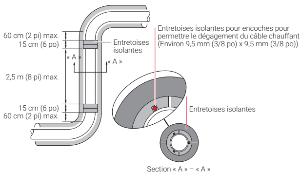
Figure 24 : Pompes
