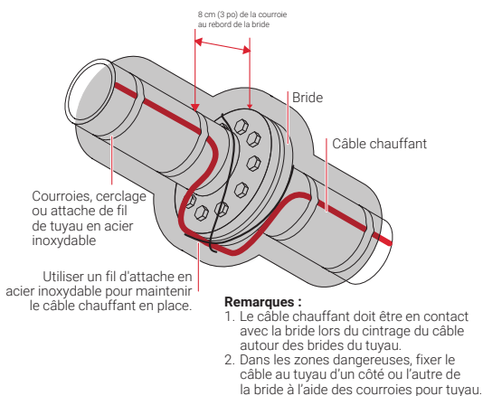
Figure 20 : Brides
