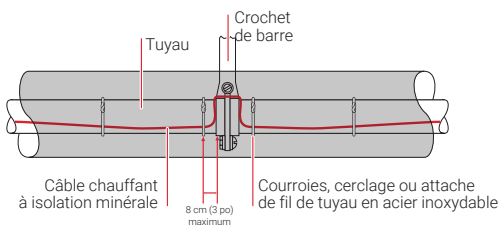
Figure 20 : Brides
