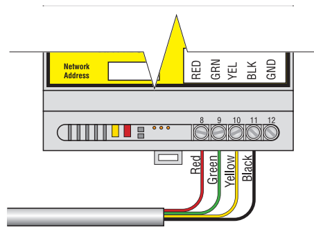
Figure 6. Sensing Cable Connections
