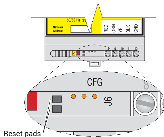
Figure 8. Reset Pads
