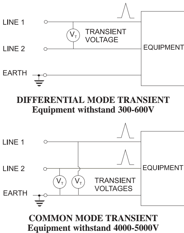
Figure 5. Typical Equipment Withstand
