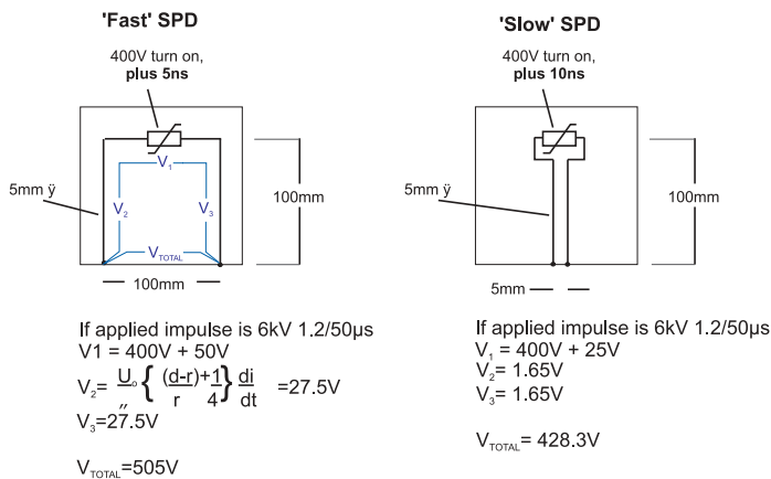
Figure 8. Speed of response is less important than let-through voltages
