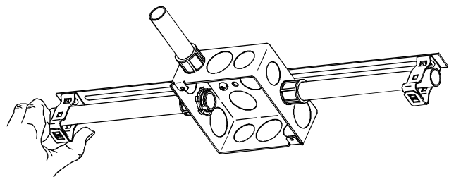
Step 3 - Finger snap clips closed around conduit.
