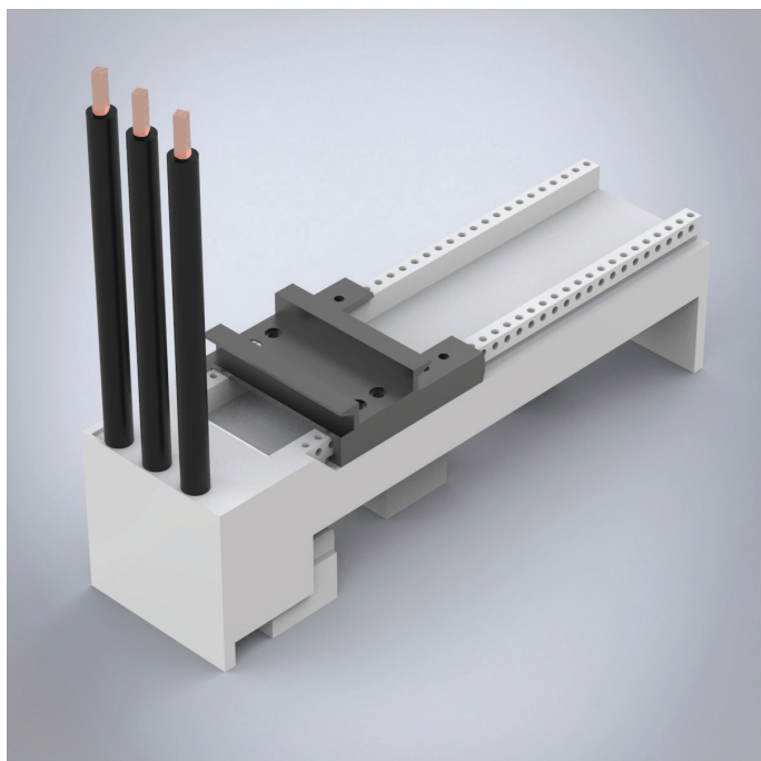
Busbar adapter with one mounting rail, pre-fitted with cables 10 mm 2 .
