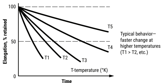
Fig. 4. Tensile elongation versus time and temperature
