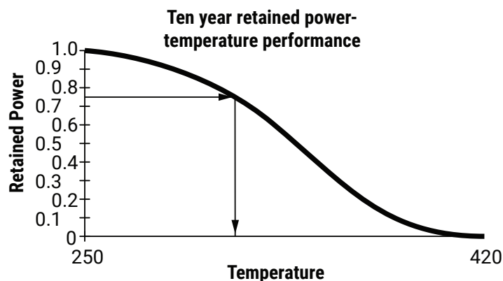
Fig. 14. Ten-year retained-power temperature performance curve
