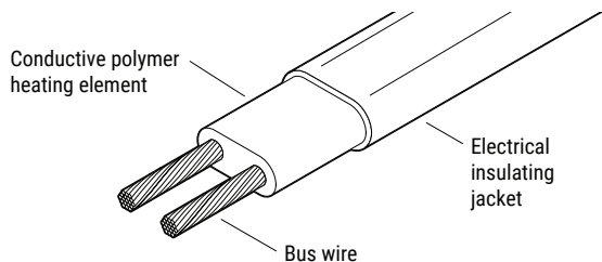
Fig. 1. Typical construction of a basic self-regulating heating-cable device
