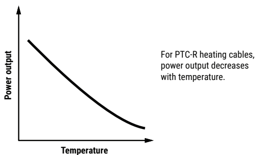
Fig. 2. Resistivity versus temperature
