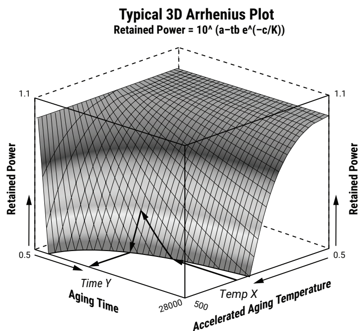
Fig. 12. Typical three-dimensional Arrhenius plot
