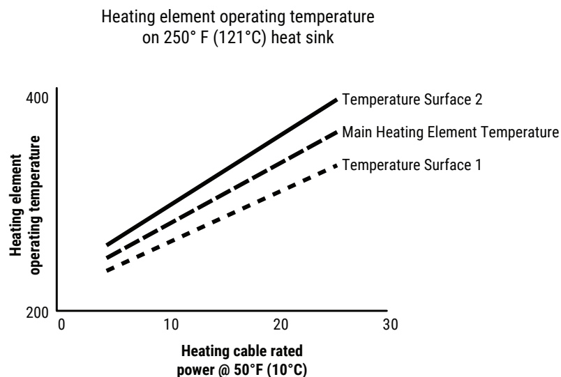
Fig. 11. Heating-element temperature (typical) versus heat-sink temperature
