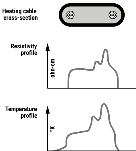
Fig. 7. Effect of nonuniform resistivity on internal temperature
