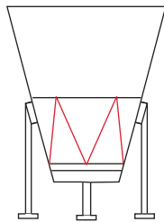
Fig. 5 Heating cable arrangement on a truncated cone
