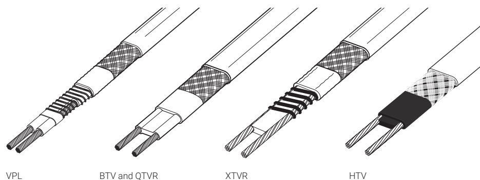
Fig. 1 Self-regulating heating cables
