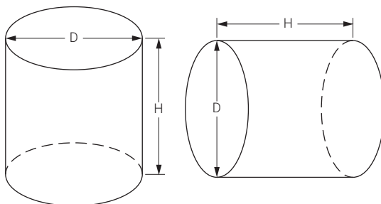
Fig. 7 Cylinder surface areas
